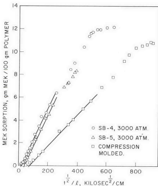
Fig. 13. Sorption of methyl ethyl ketone vapor at 25°C and 50 mm Hg pressure by polystyrene glasses vitrified at (O,Δ) 3000 atm and (□) compression-molded control.
